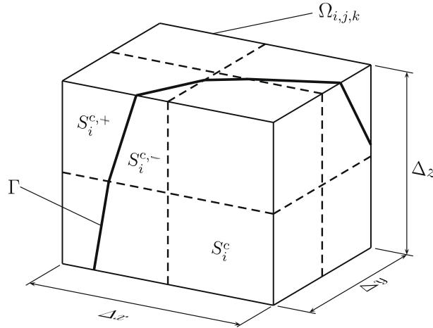
Fig. 10. Piecewise linear representation of the intersections between the boundary of control volume \Omega_{i,j,k} and the interface \Gamma . The parts of the surface bounded by the dashed lines are the inner faces of cells around node (i,j,k) as shows in Fig. 3.
