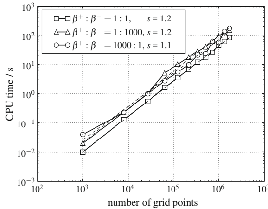
Fig. 13. CPU times for solving the resulting set of linear equations of example 2 as a function of the total number of grid points and the ratio of the coefficient \beta^+/\beta^- . The scaling factors s has been evaluated using a linear least square fit.
